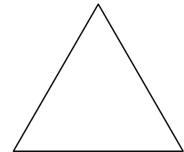
Equilateral Triangle
